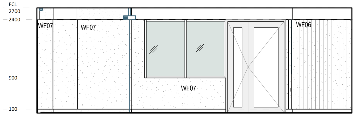
2 ELEVATION DETAIL 60-030 1 : 50
