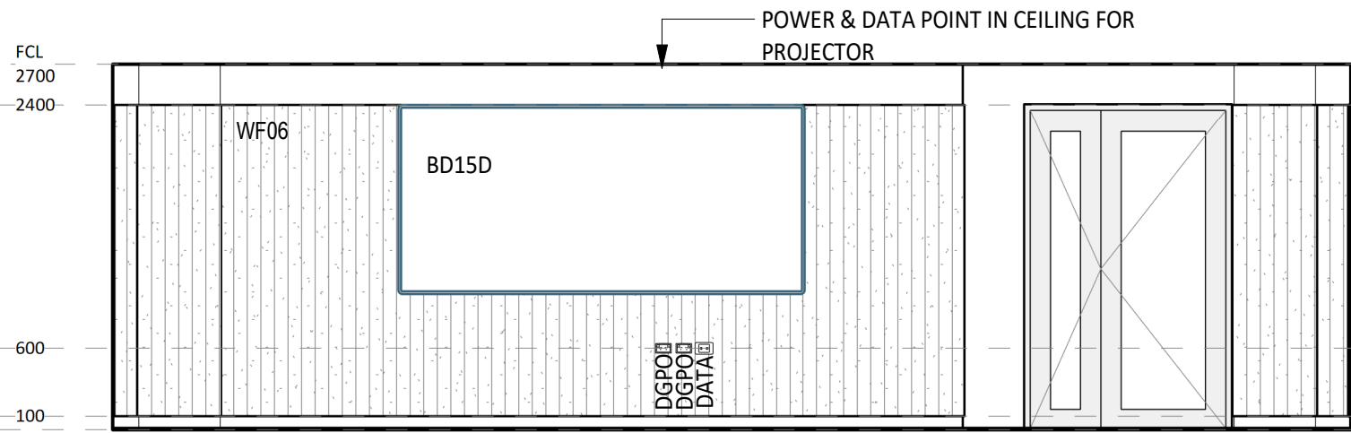
3 ELEVATION DETAIL 60-020 1 : 50
