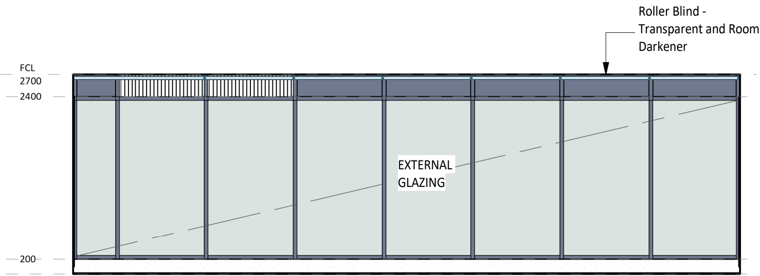
5 ELEVATION DETAIL 60-030 1 : 50
